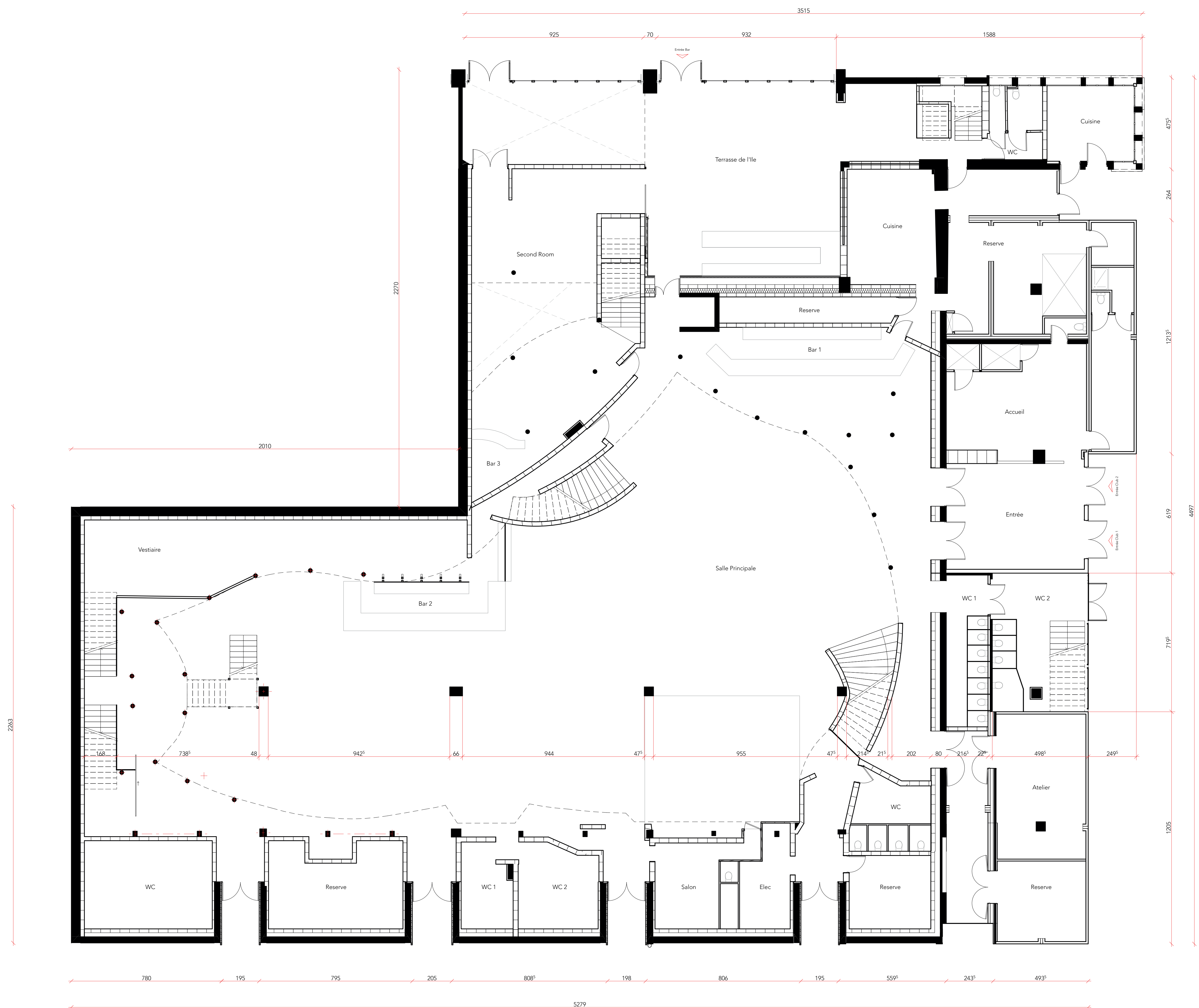
WAREHOUSE Plan RDC - 1:100
